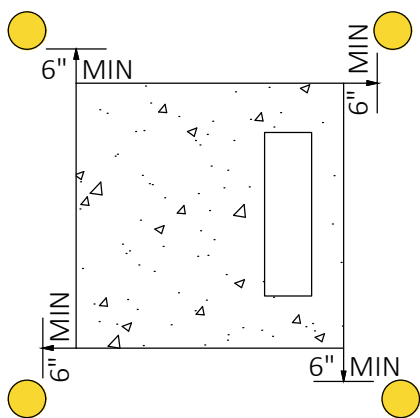
TYPICAL LAYOUT
